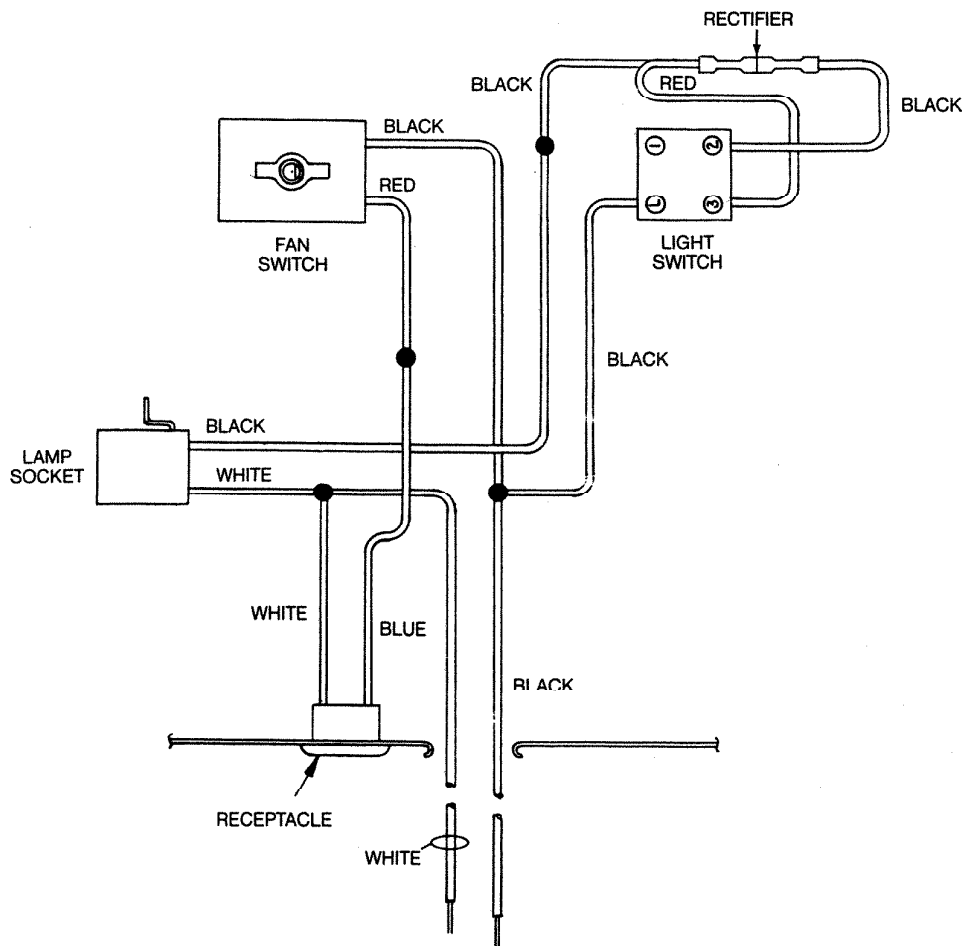
WIRING DIA. FOR MODEL NN-8300
