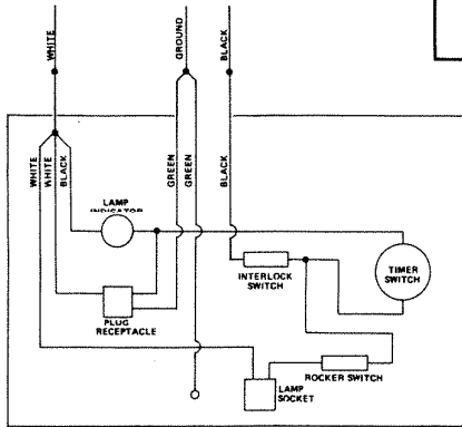
40 SERIES WIRING DIAGRAM
